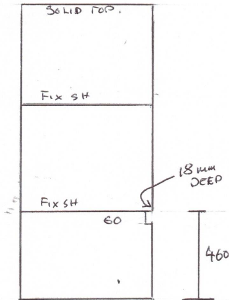
CAB 23 SIDE VIEW FLIP CUT OUT.
