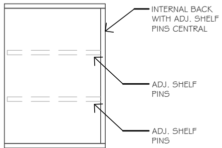
DETAIL ENDS
