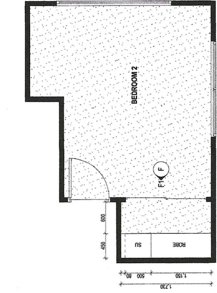
F BED 2 ROBE DETAIL PLAN SCALE: 1:50
