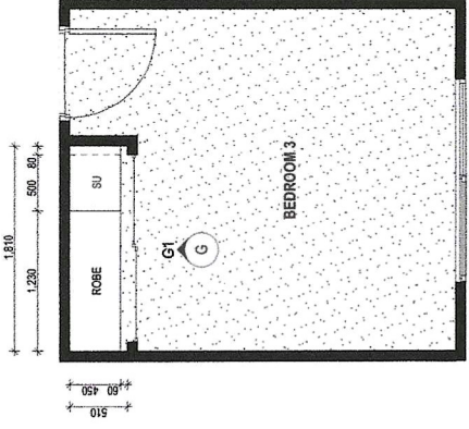
G BED 3 ROBE DETAIL PLAN SCALE: 1:50
