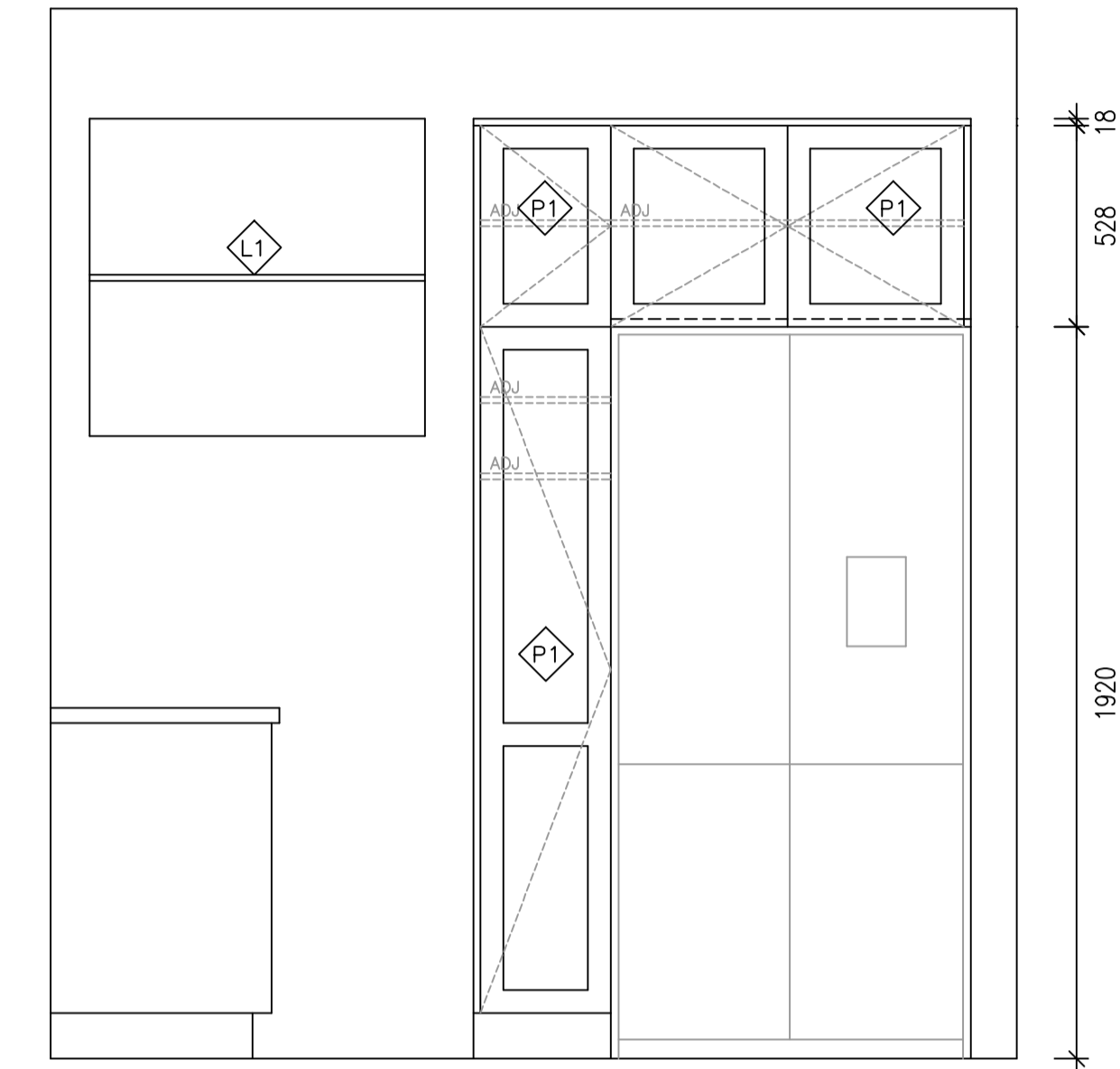
ELEVATION D
