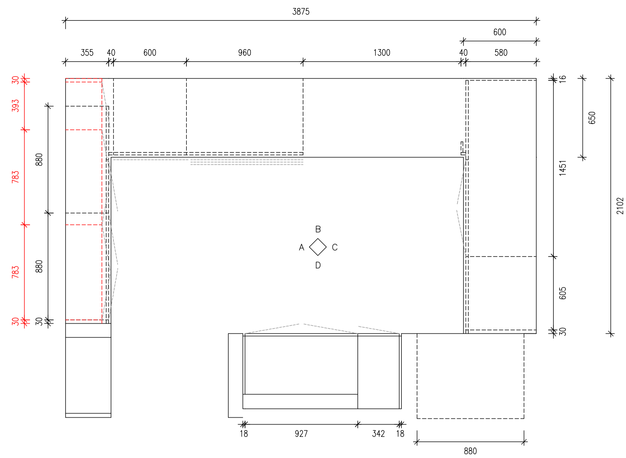
PLAN VIEW
