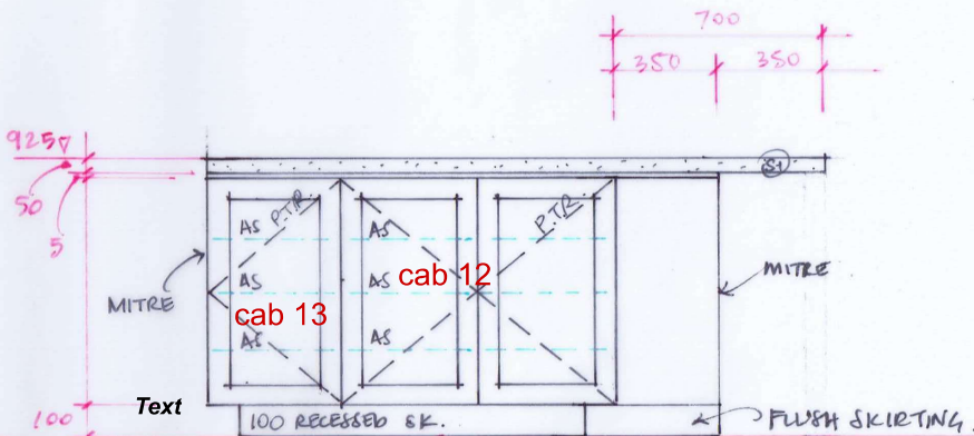
ISLAND BENCH - EAST ELEV. 1:20
