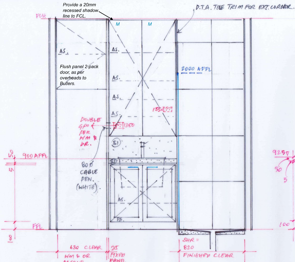
POWDER ROOM/LAUNDRY- EAST ELEVATION
