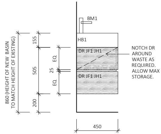
02 1:25 VANITY ELEVATION DETAIL
