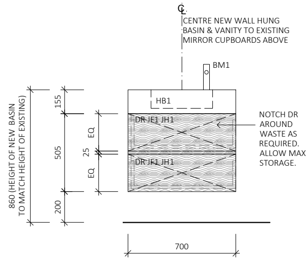
01 1:25 VANITY ELEVATION DETAIL
