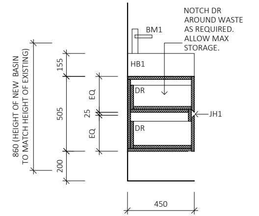
03 1:25 VANITY SECTION DETAIL
