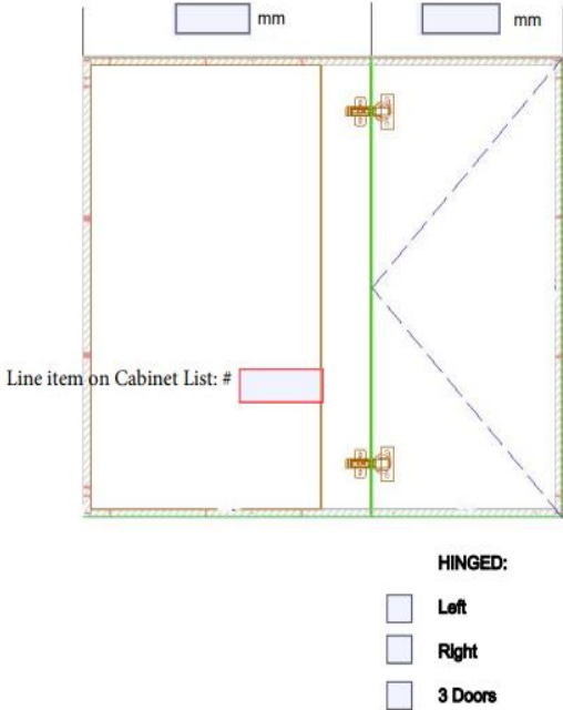
BLIND CORNER CABINET DETAIL
