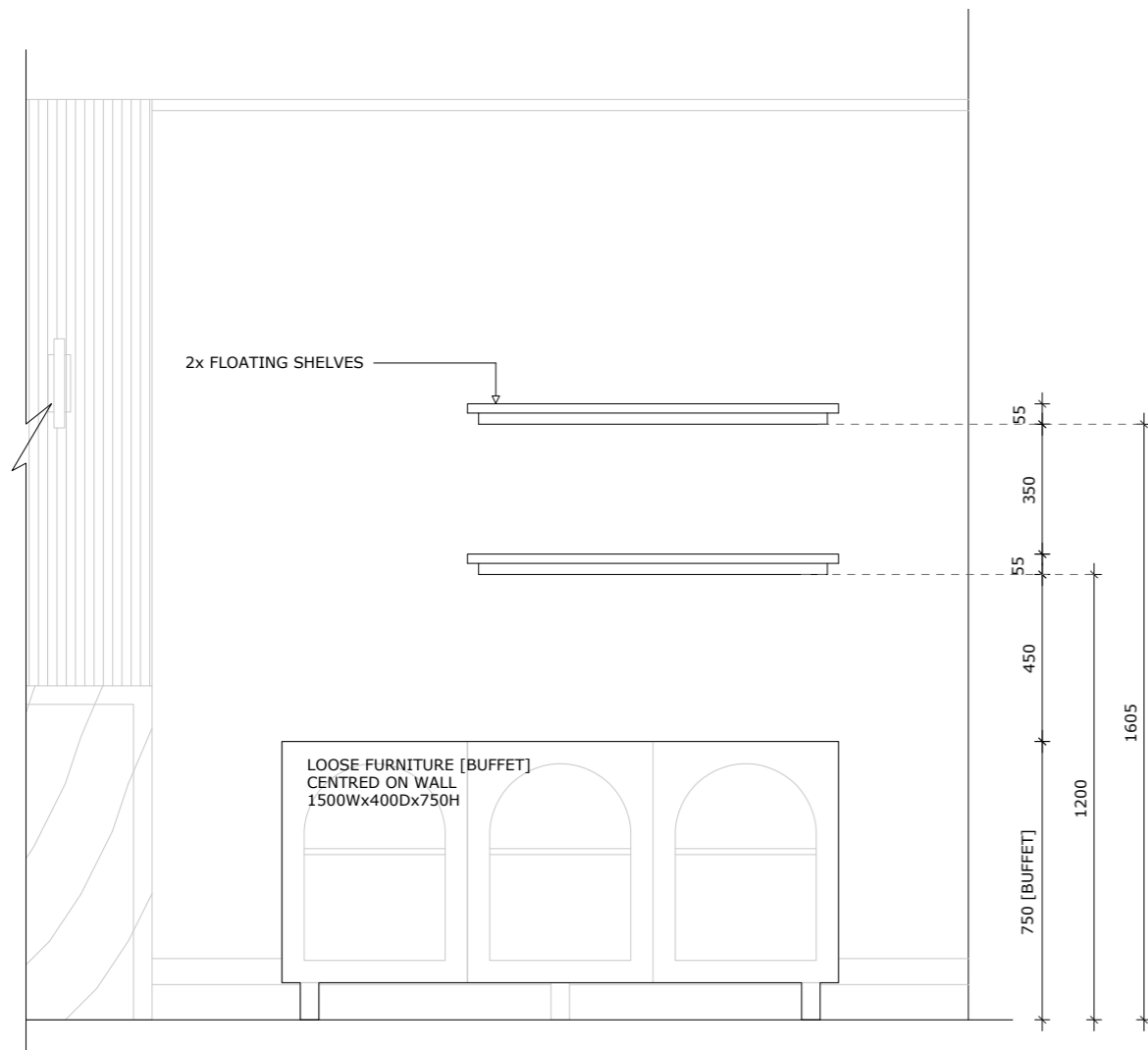
E-01 ELEVATION 01 - FLOATING SHELVES A160 Scale 1:20 @ A3
