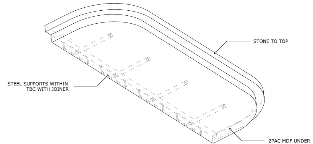
I-01 ISOMETRIC VIEW NTS
