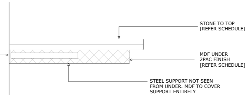
S-01 SECTION 01 - FLOATING SHELVES A160 Scale 1:5 @ A3
