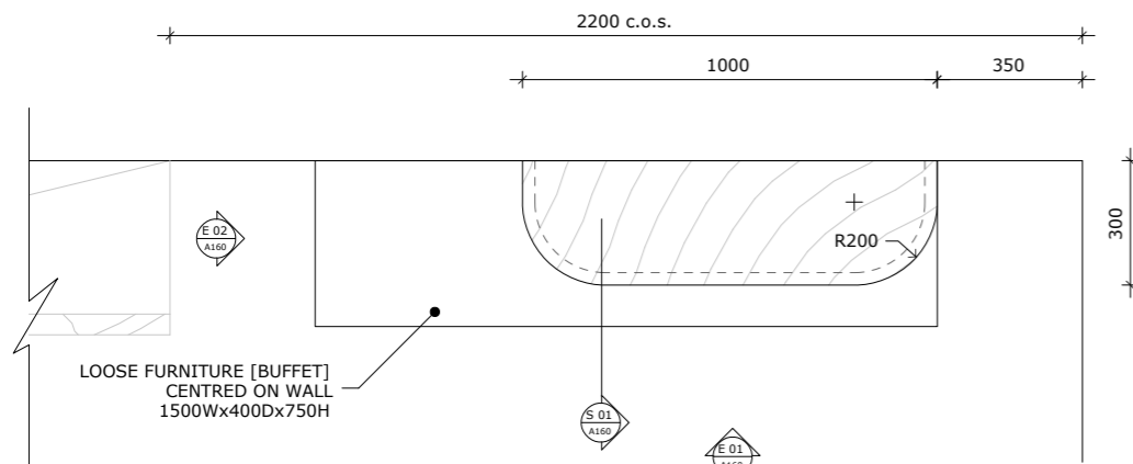
P-01 PLAN - FLOATING SHELVES Scale 1:20 @ A3
