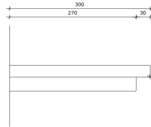
E-02 ELEVATION 02 - FLOATING SHELVES A160 Scale 1:5 @ A3
