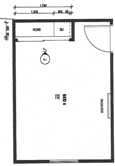
1 BEDROOM 4 ROBE DETAIL PLAN SCALE: 1:50
