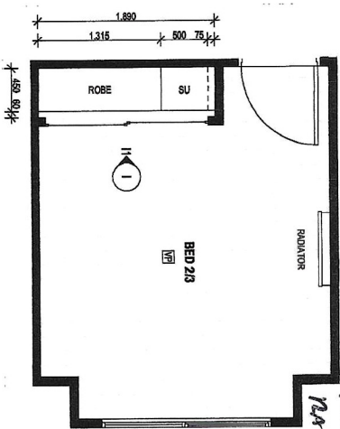
1 BEDROOM 2/3 ROBE DETAIL PLAN SCALE: 1:50
