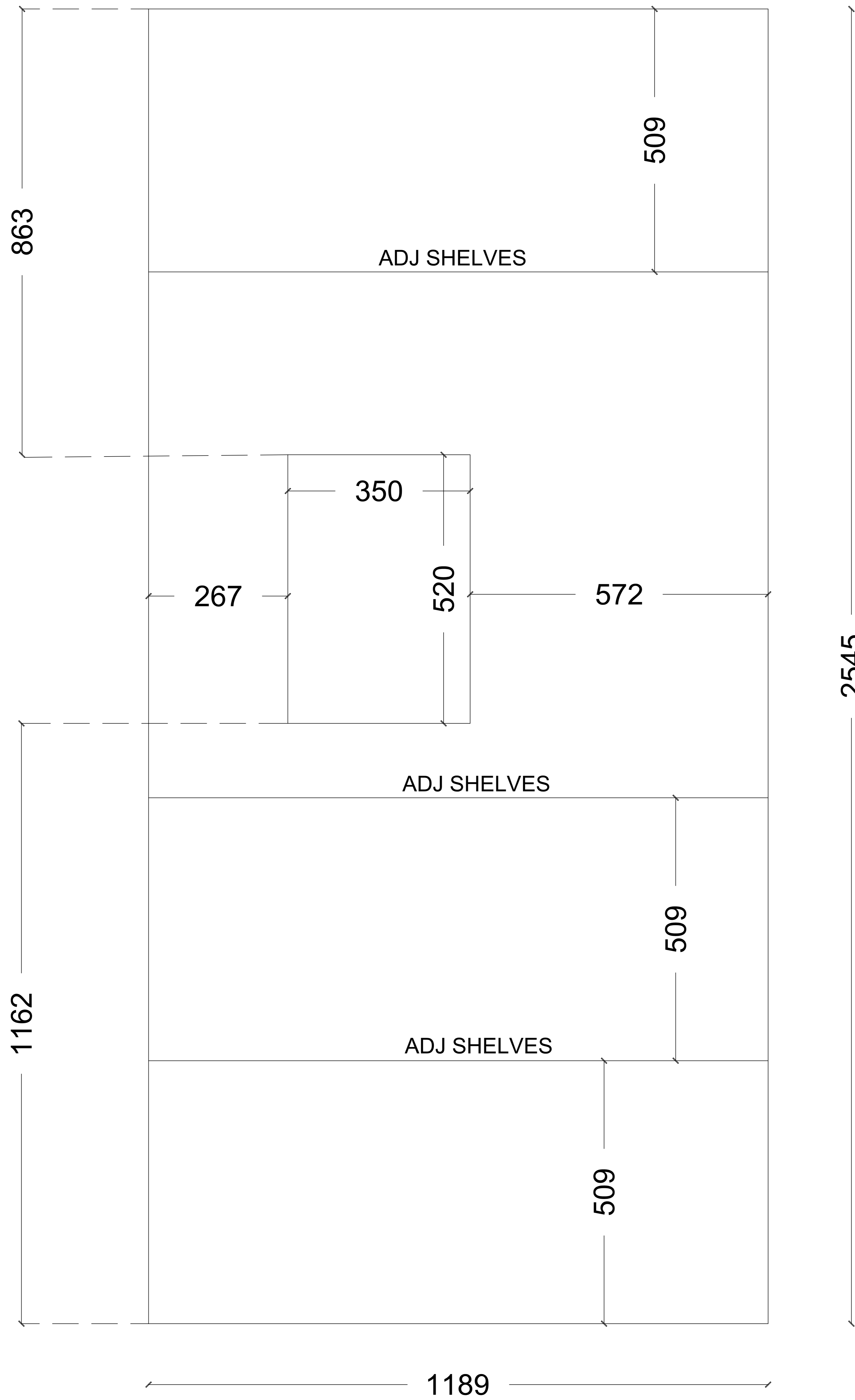
Cab # 4 Back panel cutout
