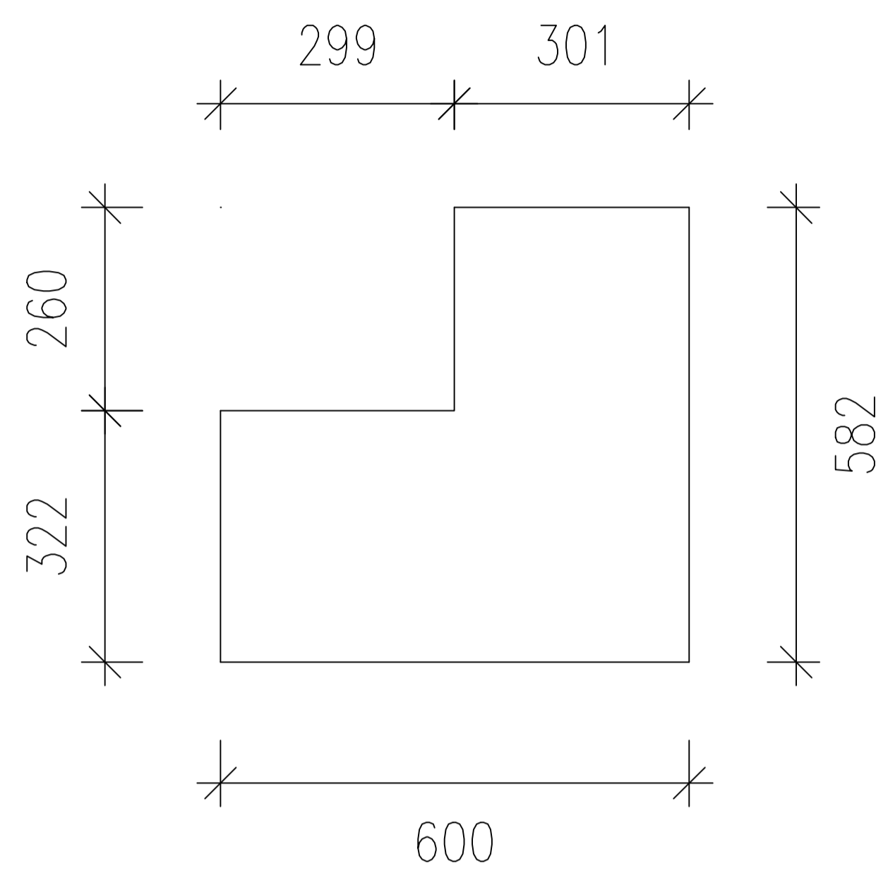
BASE CUPBOARD PLAN
