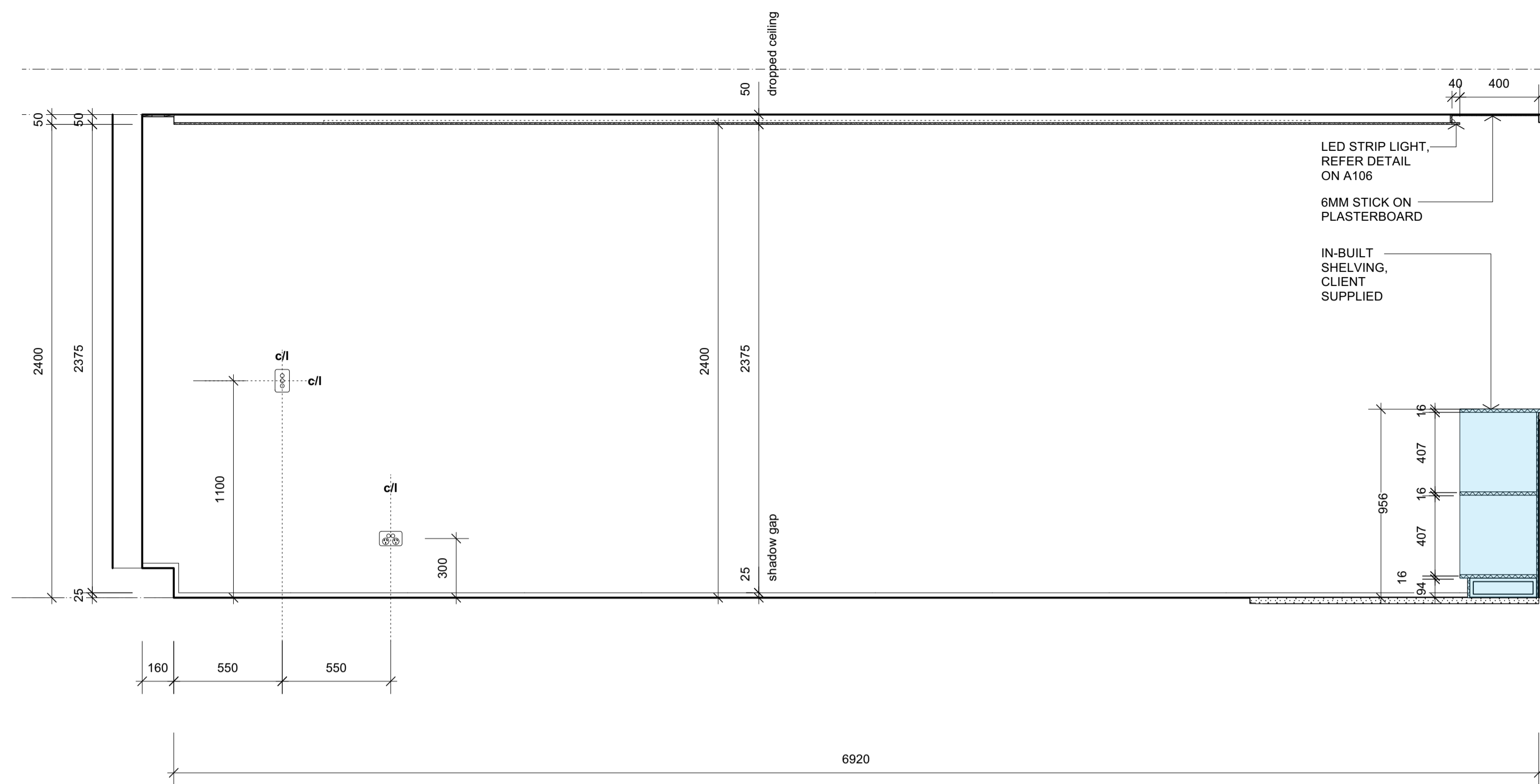
1 PROPOSED ELEVATION 1 Scale: 1:20
