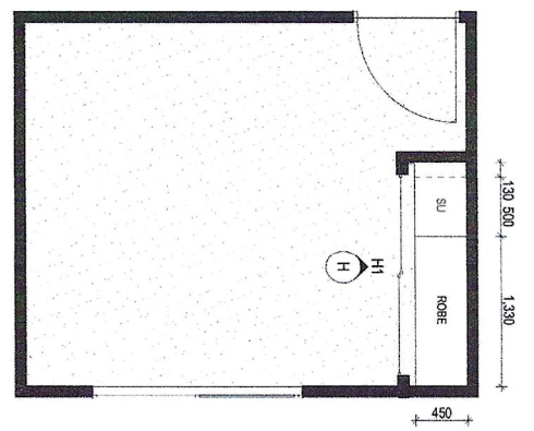
H BED 3 ROBE DETAIL PLAN SCALE: 1:50
