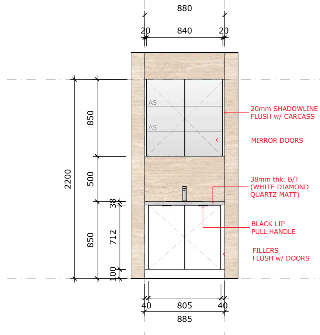
A :: VANITY FRONT ELEV. 002 scale: 1=25mm
