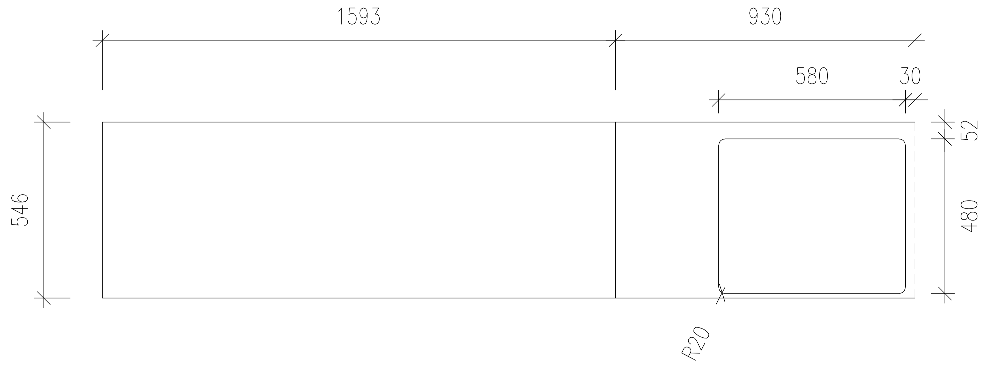
18mm MRMDF Satin White Substrate
