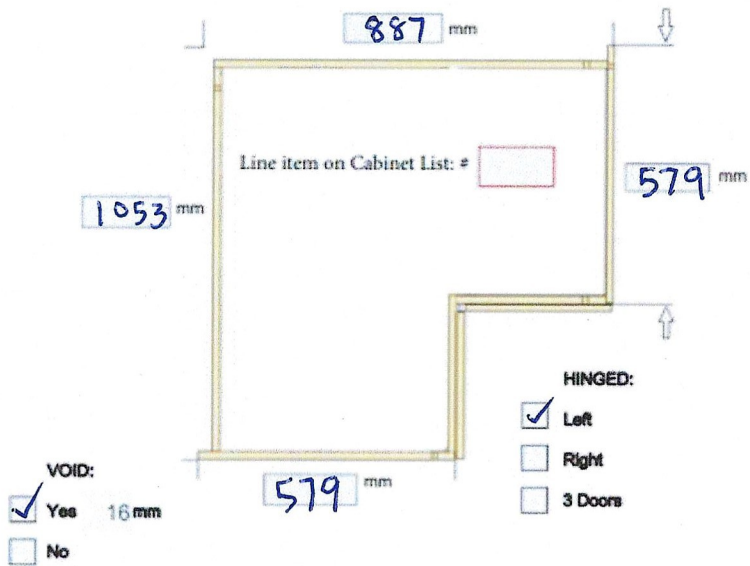
CORNER CABINET DETAIL
