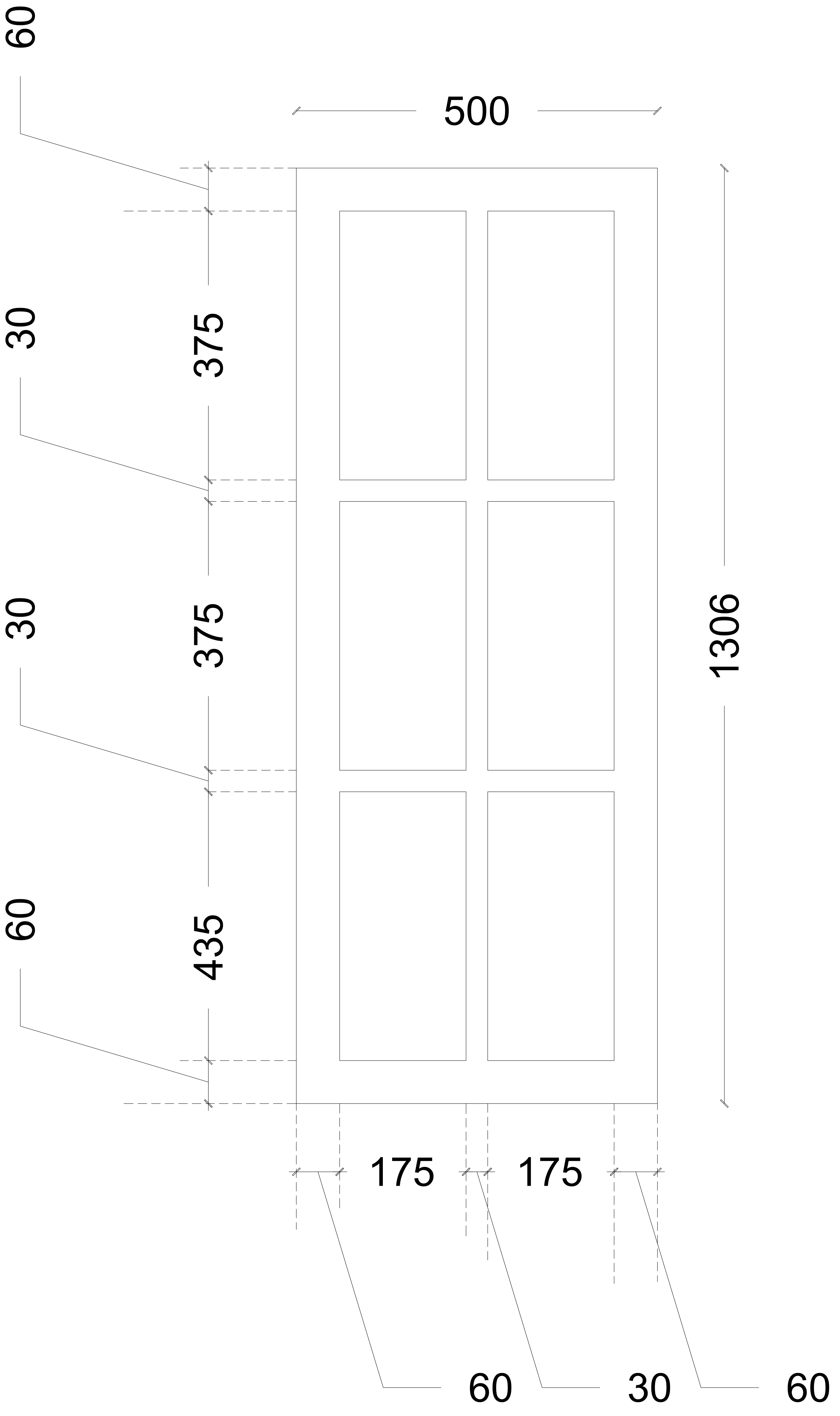
Glass Door Details
